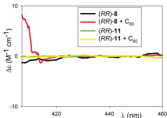
Fig. 5 CD spectra of macrocycle ( RR -8 (10 \mu M) with C_{60} (40 \mu M) and without C_{60} in toluene at 25 °C. CD spectra of the macrocycle ( RR -11 (100 \mu M) with C_{60} (400 \mu M) and without C_{60} in toluene at 25 °C for comparison.
