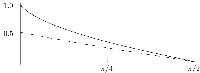
FIGURE 1. Analysis of the estimate for a wedge, 0 < \theta < \pi/2 .
